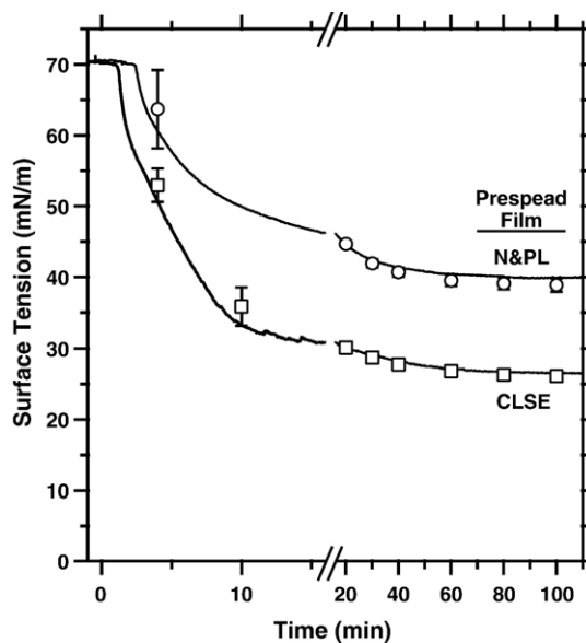
Fig. 5. Adsorption of N&PL vesicles to prespread films with and without the hydrophobic surfactant proteins. Experiments were performed at 37 ^{\circ} C by injecting 100 \mu l vesicles of N&PL into a well-stirred subphase (150 mM NaCl, 1.5 mM CaCl 2 , 10 mM HEPES pH 7.0) to a final concentration of 100 \mu M phospholipid below a preexisting film containing either N&PL or CLSE at 1.02 \mu mol/m 2 phospholipid. Curves are representative of at least three experiments. Symbols indicate the mean \pm S.D. at selected times.
