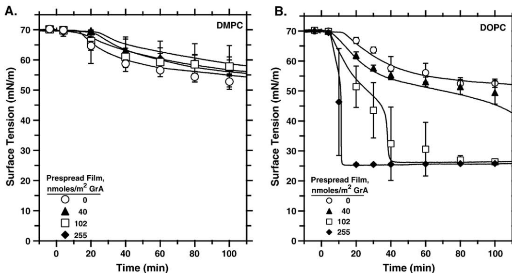
Fig. 6. Adsorption of phospholipid vesicles to preformed phospholipid films containing different amounts of GrA. Experiments were performed at 37 °C by injecting 150 \mu l of lipid vesicles without GrA to a final concentration of 150 \mu M lipid into a well stirred subphase (150 mM NaCl, 10 mM HEPES pH 7.0) below a prespread film containing 1.02 \mu mol/m 2 phospholipid with different amounts of GrA. Curves are representative of at least three experiments. Symbols give the mean \pm S.D. at selected times. (A) DMPC. (B) DOPC.
