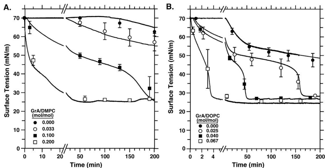
Fig. 4. Adsorption to the air–water interface of phospholipid vesicles with different amounts of GrA. Experiments were performed at 150 \mu M phospholipid in buffered saline (150 mM NaCl, 10 mM HEPES pH 7.0) at 37 ^{\circ} C. Ratios of GrA/DOPC are mole/mole. Curves are representative of at least three experiments, with mean \pm S.D. shown at selected times. (A) DMPC. Data for GrA/DMPC of 0.02 and 0.07, which are omitted for clarity of presentation, fit in the sequence of curves according to the dose of GrA. (B) DOPC. Omitted data for GrA/DOPC of 0.02, 0.04, 0.10 similarly fit in the sequence of curves according to the dose of GrA.
