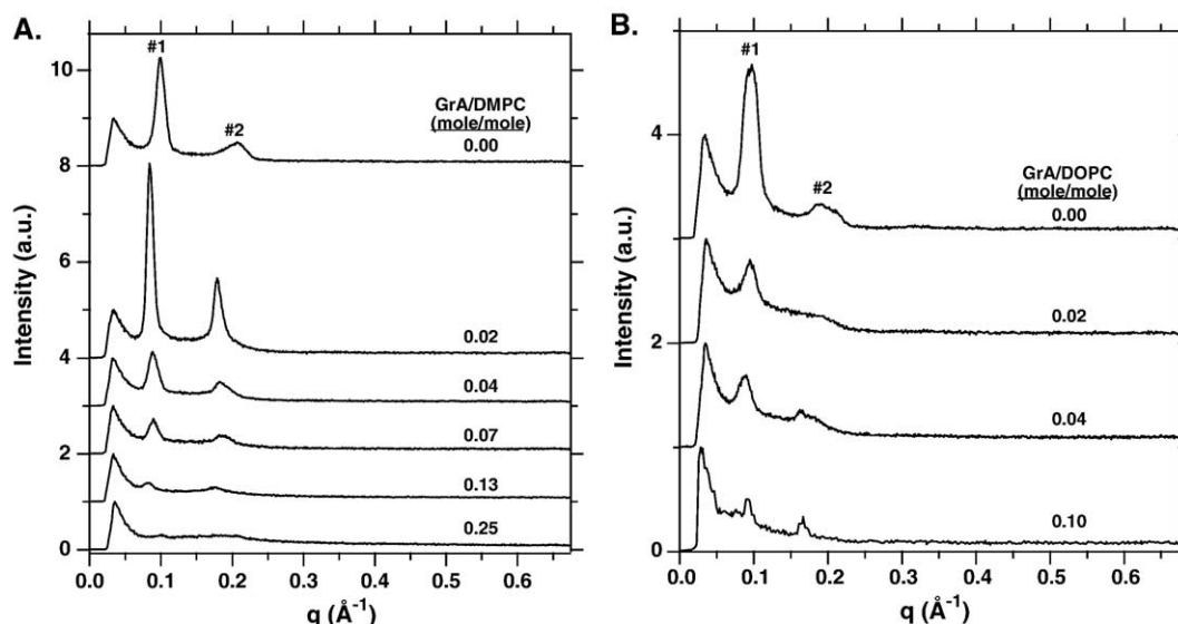
Fig. 1. SAXS from dispersed samples of phospholipid with different amounts of GrA. Profiles were obtained with a constant phospholipid concentration of 30 mM in buffered saline (150 mM NaCl, 10 mM HEPES pH 7.0) at 37 °C. The first and second order diffraction peaks are labeled for phospholipid without GrA. For clarity of presentation, the curves for the different experiments are each shifted by a constant value of intensity. (A) DMPC. (B) DOPC.
